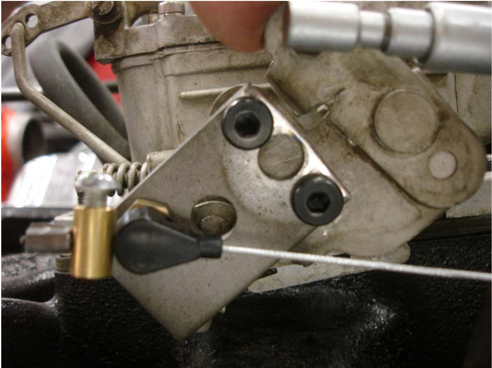
Carb linkage at full throttle
